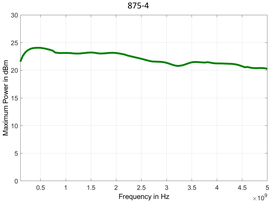
Figure 3: Maximum Output Power
