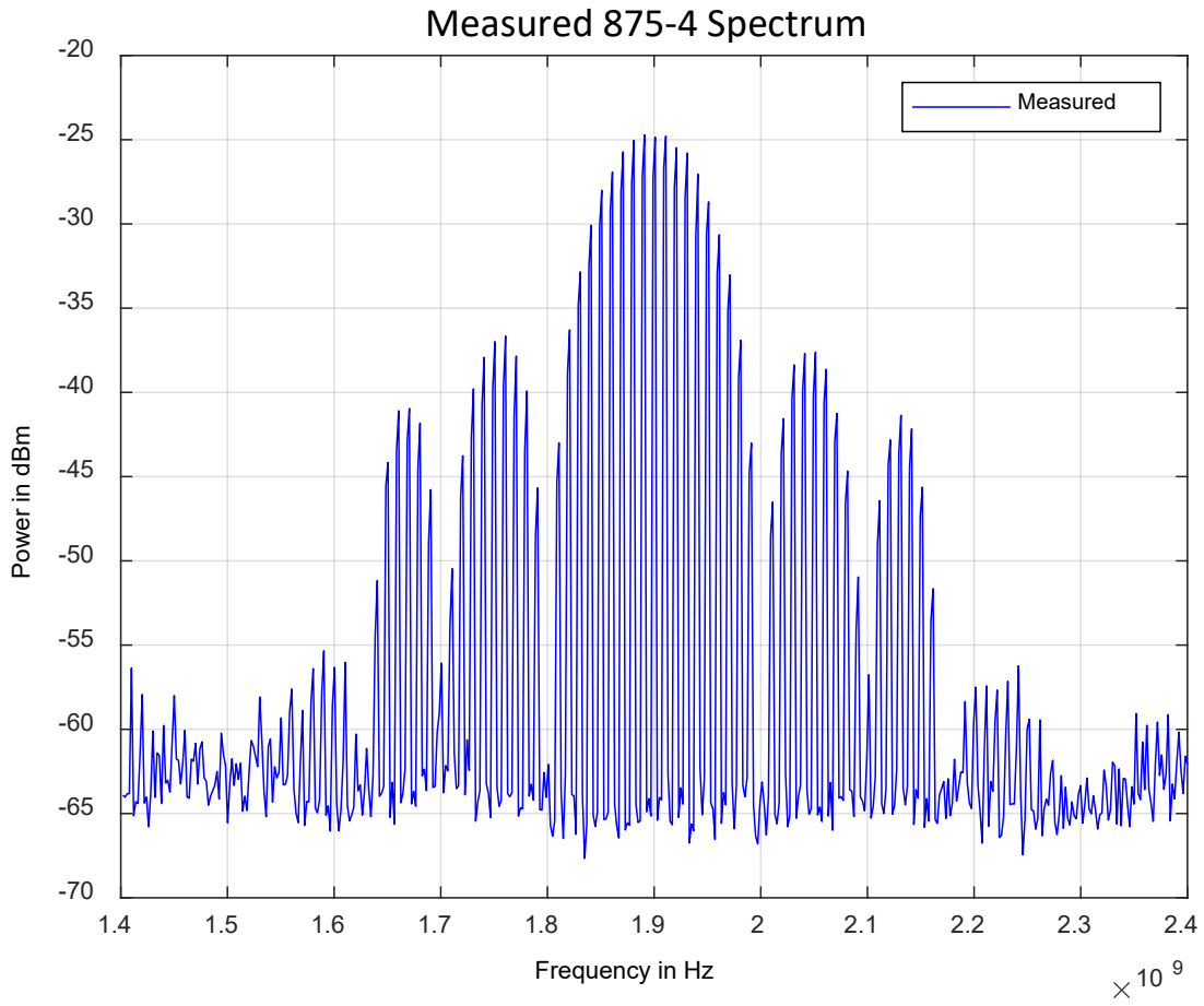
Figure 13: Pulse modulation (10 MHz rate, 10 ns pulse width)
