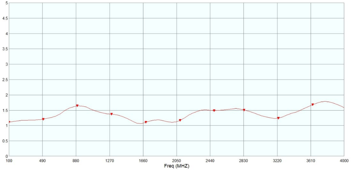
Figure 20: Typical VSWR (875-12 & 875-20)
